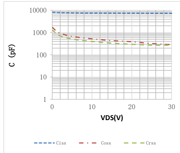
Fig.2 Capacitance Characteristics
