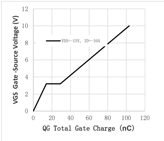
Fig.1 Gate-Charge Characteristics
